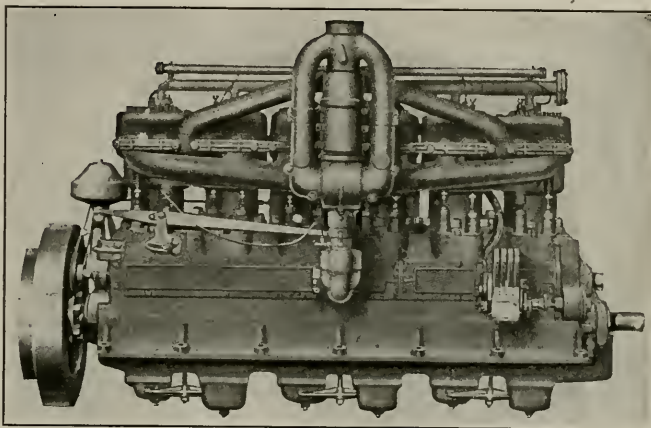
7¼ BY 9 INS. SIX-CYLINDER ENGINE, VALVE SIDE.
